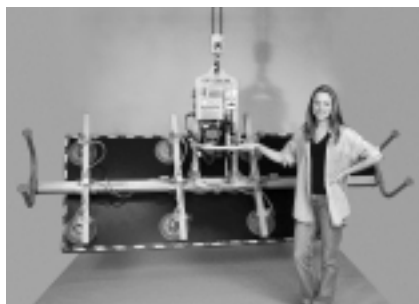
Eight Pad Electric Powered Vacuum Lifter with Powered Tilt
