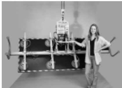
Eight Pad Electric Powered Vacuum Lifter with Powered Tilt
