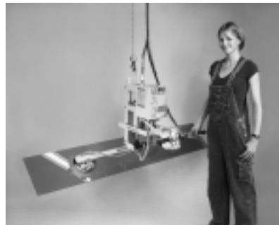
Two Pad Air Powered Air Balancer Vacuum Lifter with Powered Tilter
