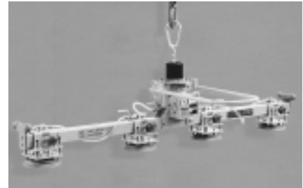
Self-Powered Mechanical Vacuum Lifter with Four Adjustable In-Line Vacuum Pads
