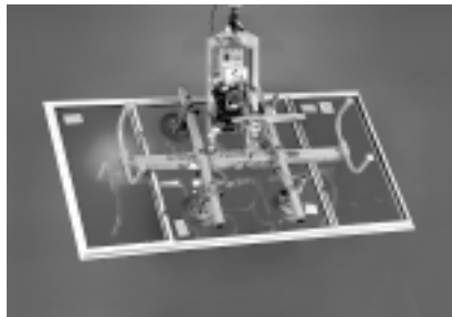
Four Pad Electric Powered Vacuum Lifter with Powered Tilt
